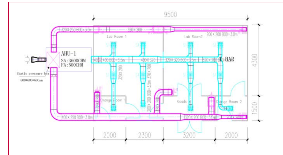
HVAC System Design
