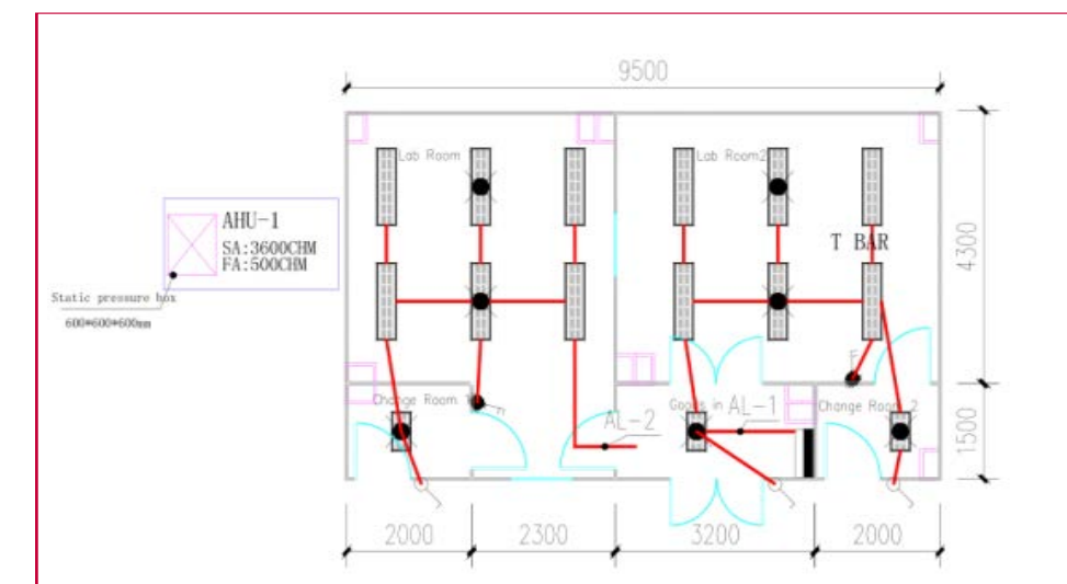
Lighting System Design
